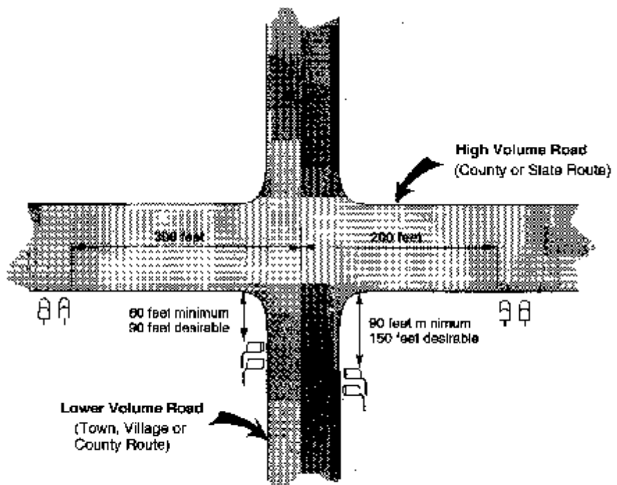
Figure 6: Mailbox location at major intersections
