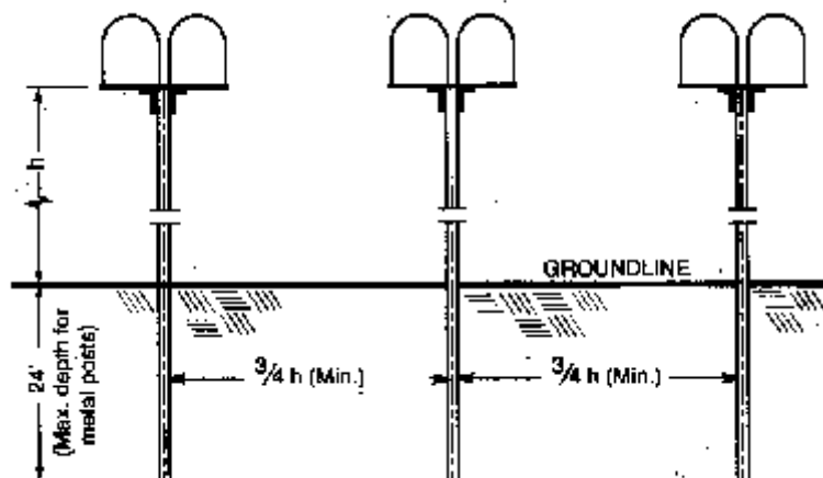
Figure 1: Spacing for multiple post installations.
