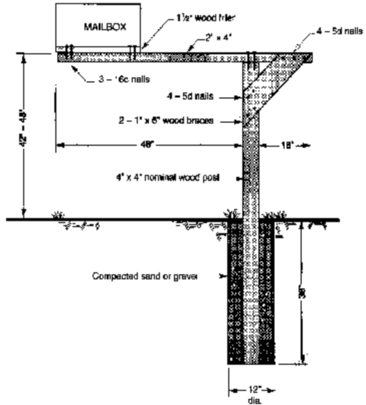
Figure 4: Example of a wood cantilever mailbox support.
